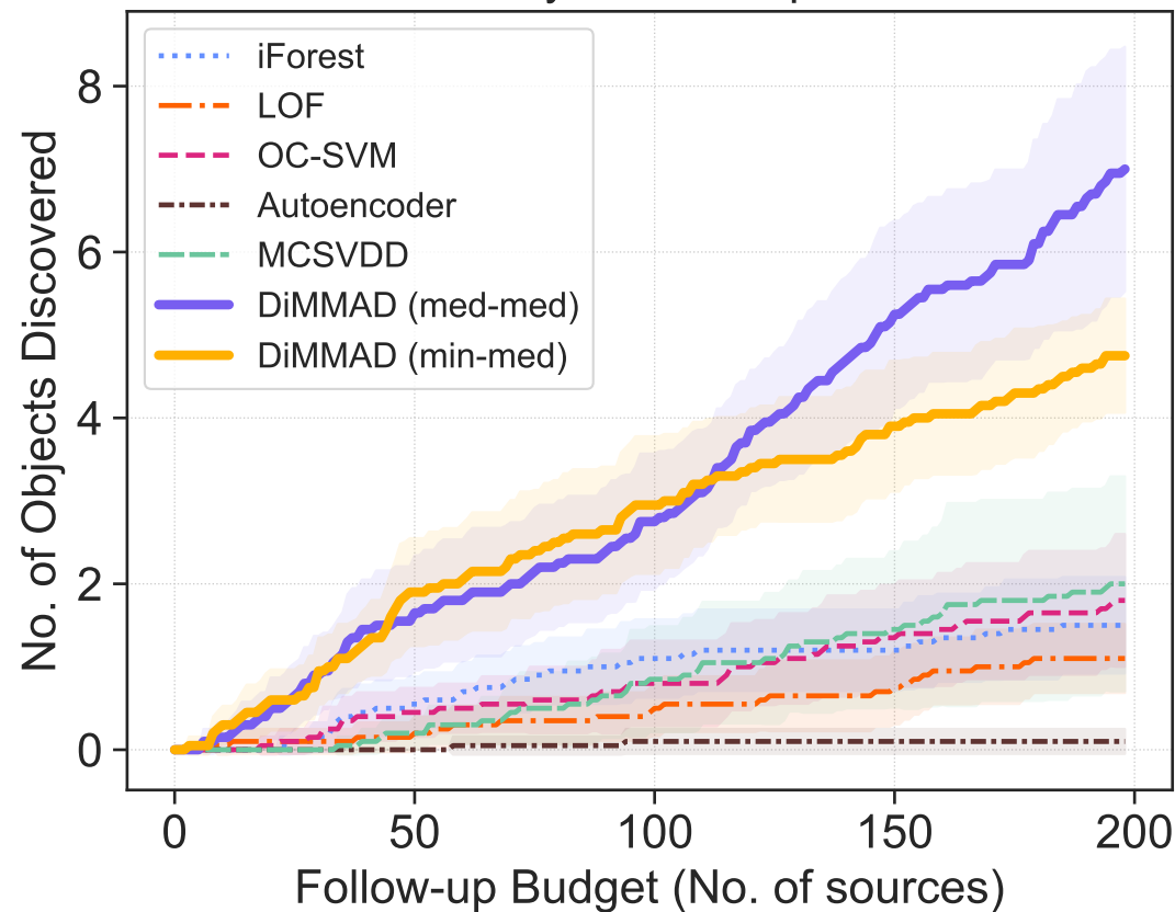
Anomaly: SNII-Templates
